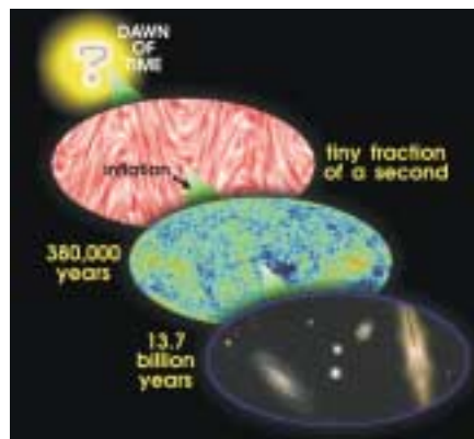
Figure 1 — Artist's concept of crucial periods in the development of the Universe according to Big Bang inflationary cosmology
