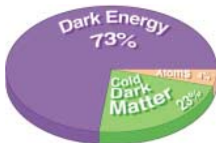
Figure 5 — Chart depicting the percentages of dark energy, dark matter, and actual matter (i.e., atoms) that must be present in order to explain the composition of the Universe via the Big Bang model
