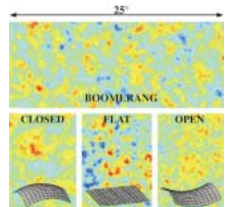
Figure 3 — The possible shapes of the Universe—closed, flat, or open—are based on how imaginary pairs of parallel lines might act. The bottom simulations represent the data that would result if each were correct, since BOOMERANG measures “hot” and “cold” spots (i.e., cosmic microwave background radiation) in the Universe. The top image depicts the actual BOOMERANG data.
