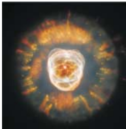
This image, nicknamed the Eskimo Nebula because of the “parka” surrounding the dying star, was captured by the Hubble Telescope in December 1999 after it was repaired. Image courtesy of NASA.
