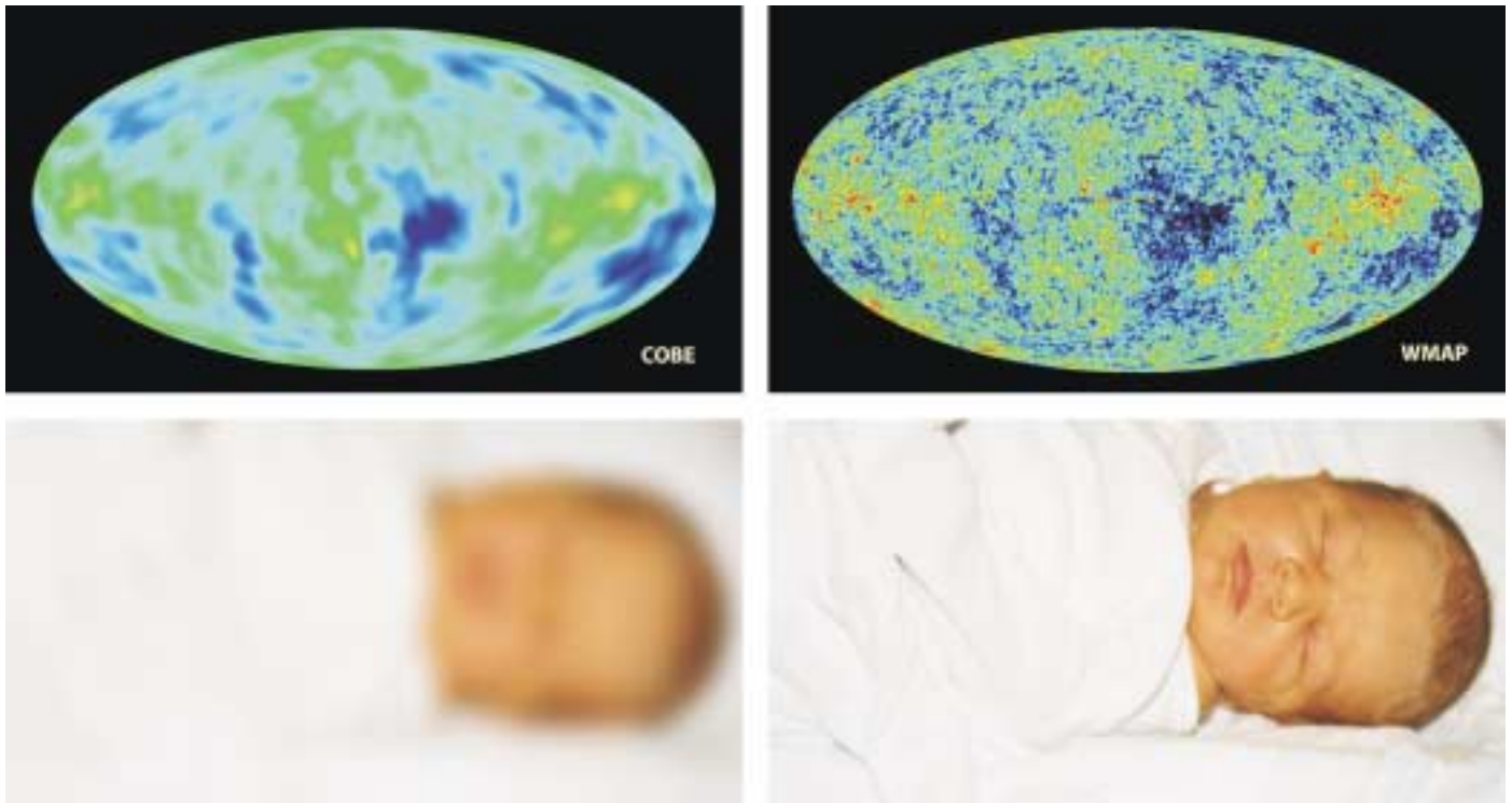
Figure 2 — Image at top left allegedly represents a “baby picture” of the Universe taken by the COBE satellite, first launched November 18, 1989. [Oval shape is a projection to display the entire sky, similar to the way the globe of the Earth can be projected as an oval.] Colors indicate “warmer” (red/yellow) and “cooler” (blue) spots. Image at top right (taken by NASA’s Wilkinson Microwave Anisotropy Probe [WMAP], launched June 30, 2001) brings the COBE picture into sharp focus, similar to refocusing a camera lens after taking an infant’s snapshot, as in examples above. The high-resolution WMAP image supposedly depicts the microwave light from 380,000 years after the Big Bang, which is said to have occurred 13.7 billion years ago. This would be the equivalent of taking a picture of an 80-year-old man or woman on the day of his or her birth. CMB images courtesy of NASA.
