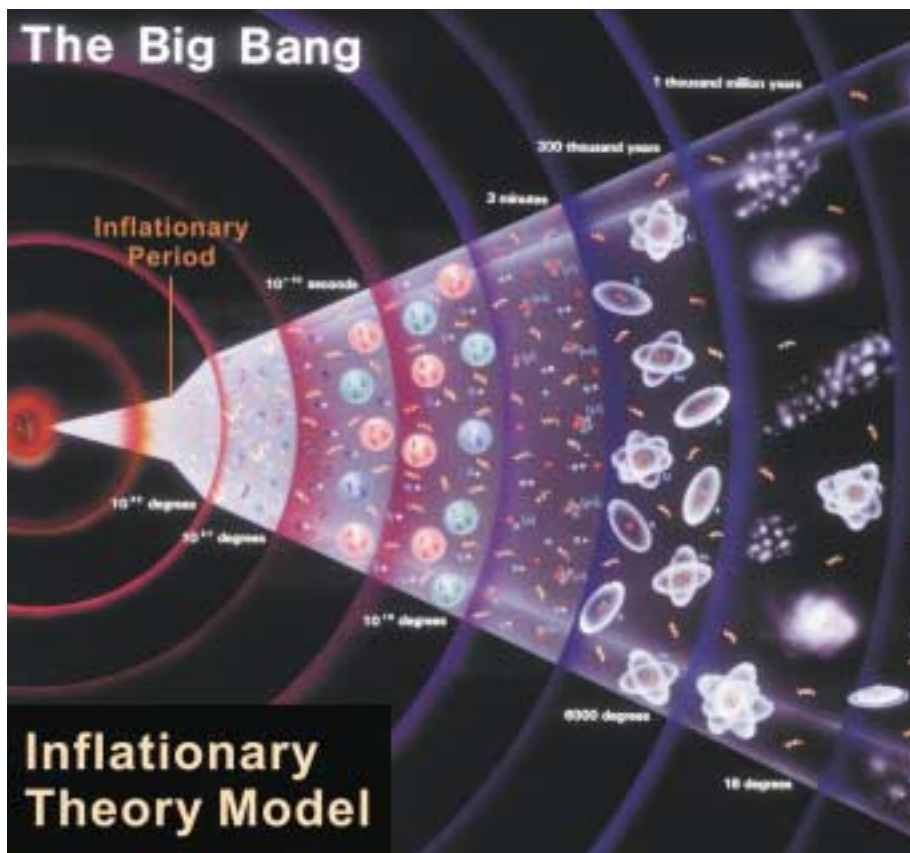
Figure 7 — Artist's depiction of the Big Bang Inflationary Model. Image courtesy of CERN.
