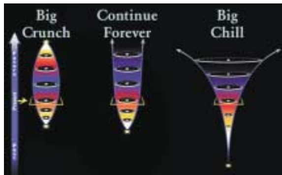
Figure — 6 Three models depicting the possible fate of the Universe from an evolutionary viewpoint. (1) In an expanding Universe, the combined gravity from the matter slows expansion. If the pull is strong enough, the expansion will stop and reverse itself, resulting in a “Big Crunch.” (2) If the gravitational forces equal the expansion forces, then the Universe theoretically will continue forever (even though expansion slows down over time). (3) If gravitational forces are not strong enough, and are overcome by expansion forces, then the Universe supposedly will continue to expand, eventually ending in a “Big Chill.”
