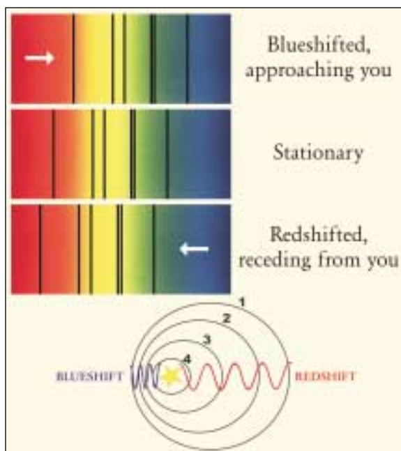
Figure 1 — Blueshift/Redshift Depiction
